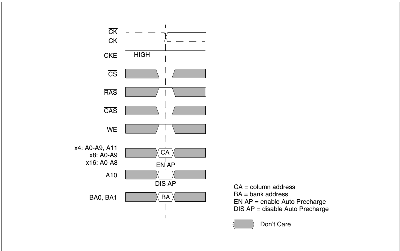
Figure 9 Read Command
